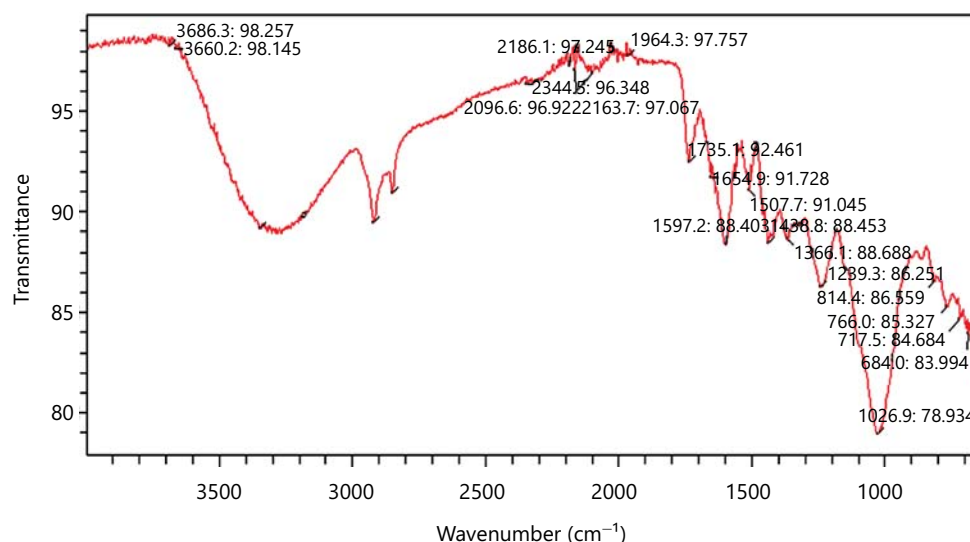
Fig. 4: FTIR spectrum of date seed powder
